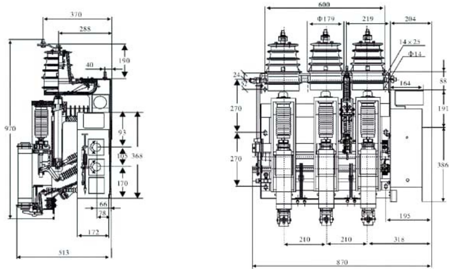
(负荷开关外形尺寸图) Drawing of load switch outline dimensions
